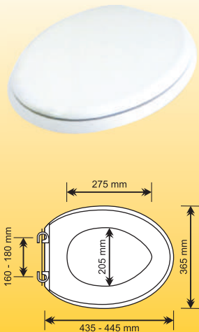
CJSC 2003 HD Heavy Duty Seat & Cover
