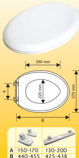
CJSC 2008 MD Medium Duty Seat & Cover
