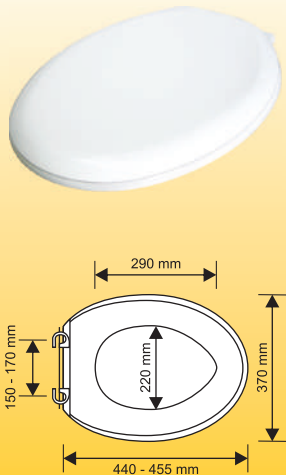
CJSC 2001 LD Light Duty Seat & Cover
